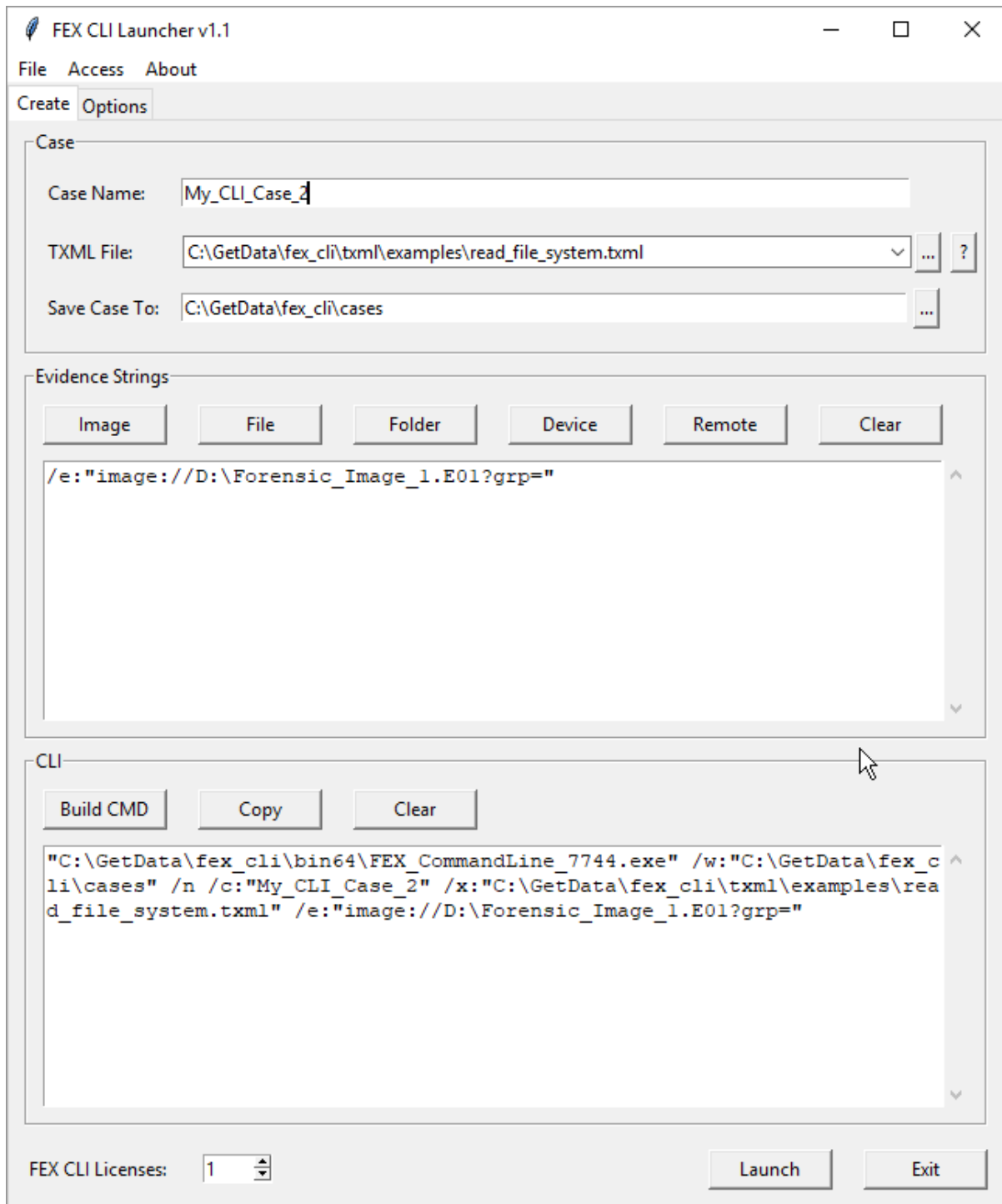
Figure 14: fex_cli_launcher.exe
